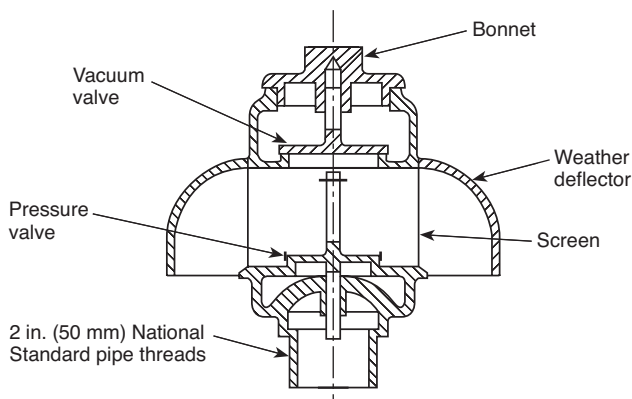
FIGURE A.3.3.32 Pressure Vacuum Vent.
